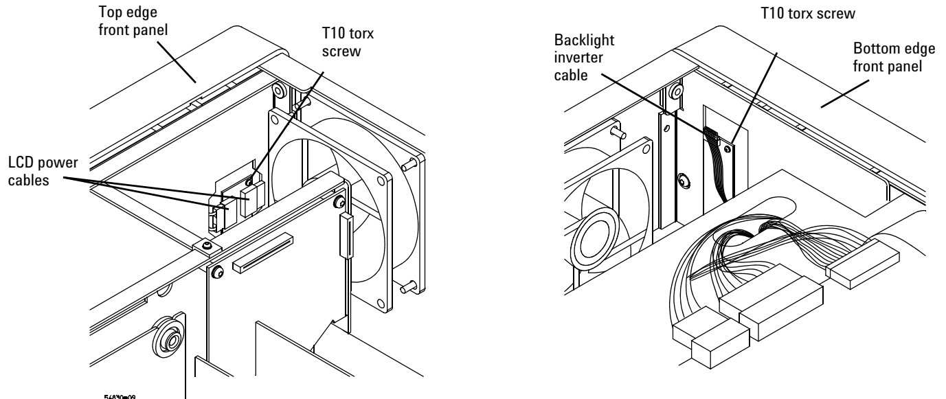
Removing the backlight inverter board
